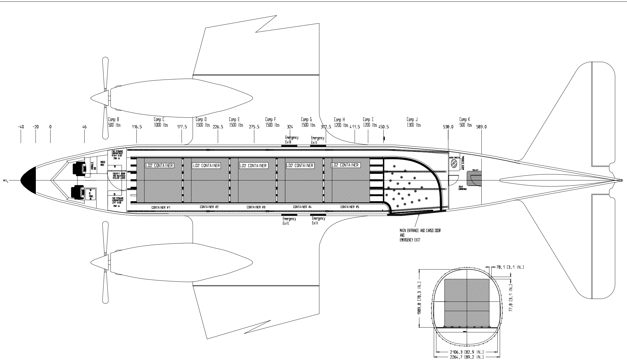
CARGO COMPARTMENT DIMENSIONS FS 450.5 TO 116.5
